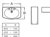
Lavabo / Pedestal / Semipedestal
